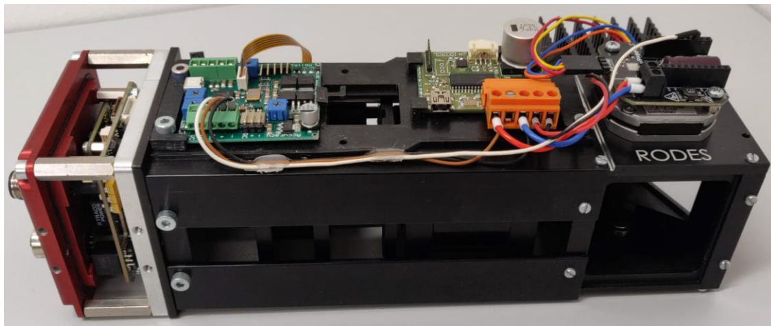
Hyperspectral LWIR camera RODES
